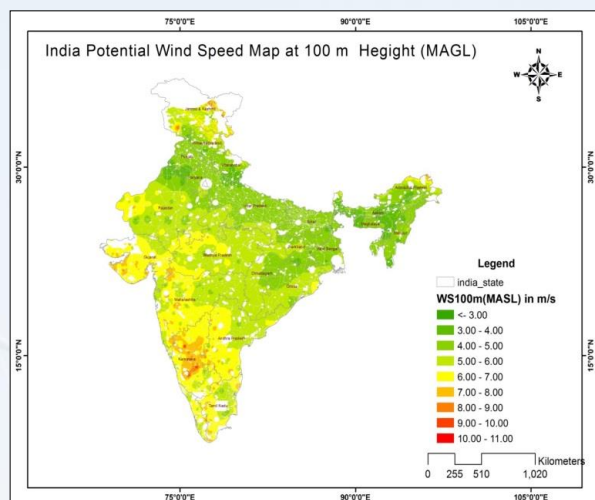
Figure 1: India Wind Speeds at 100 m Hub Height
